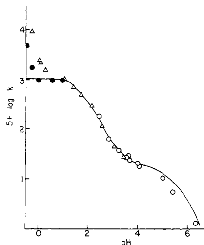
Figure 2. pH-rate profile for decomposition of 9-propylpurine-6-diazotate at 25.0°: HCl (Δ), HClO 4 (●), calculated using buffer dilution (○). The line is calculated using the derived rate constants.
