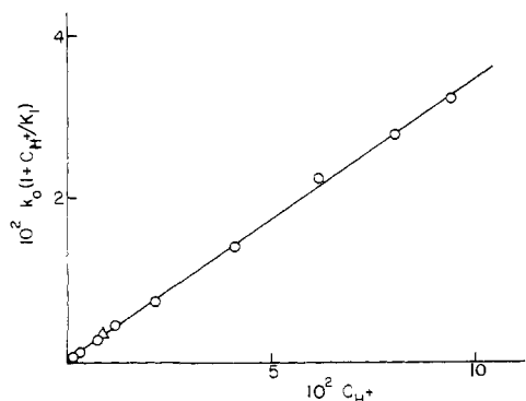
Figure 4. Determination of k_H and k_w for decomposition of 9-propylpurine-6-diazotate: HCl (O), HCl + 0.1 M NaCl ( \Delta ).
