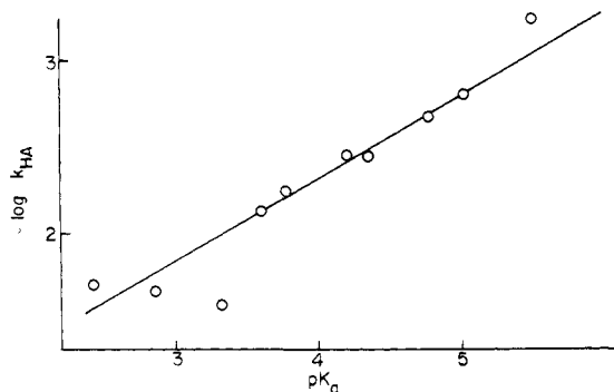
Figure 3. Bronsted plot for decomposition of 9-propylpurine-6-diazotate at 25.0°.
