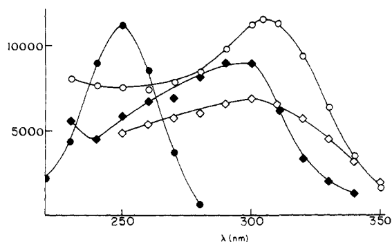
Figure 1. Spectra of 9-propylhypoxanthine (●) and 9-propylpurine derivatives: diazotate (○), diazohydroxide (◇), and protonated diazohydroxide (◆).
